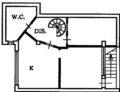
PIANO SEMINTERRATO H=2,40
